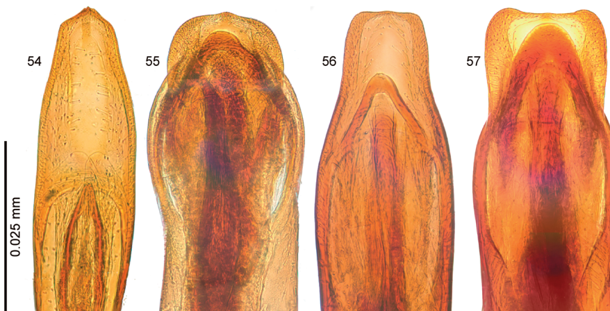
Figures 54–57 Aedeagus, apex of median lobe, ventral view. 54 , Catops hlisnikovskiyi n. sp., holotype (JRUC). 55 , C. schuelkei n. sp., holotype (MSCC). 56 , C. sasajii Nishikawa (93 km S Zhouzhi, JRUC). 57 , C. smetanai n. sp., holotype (MPEC).
