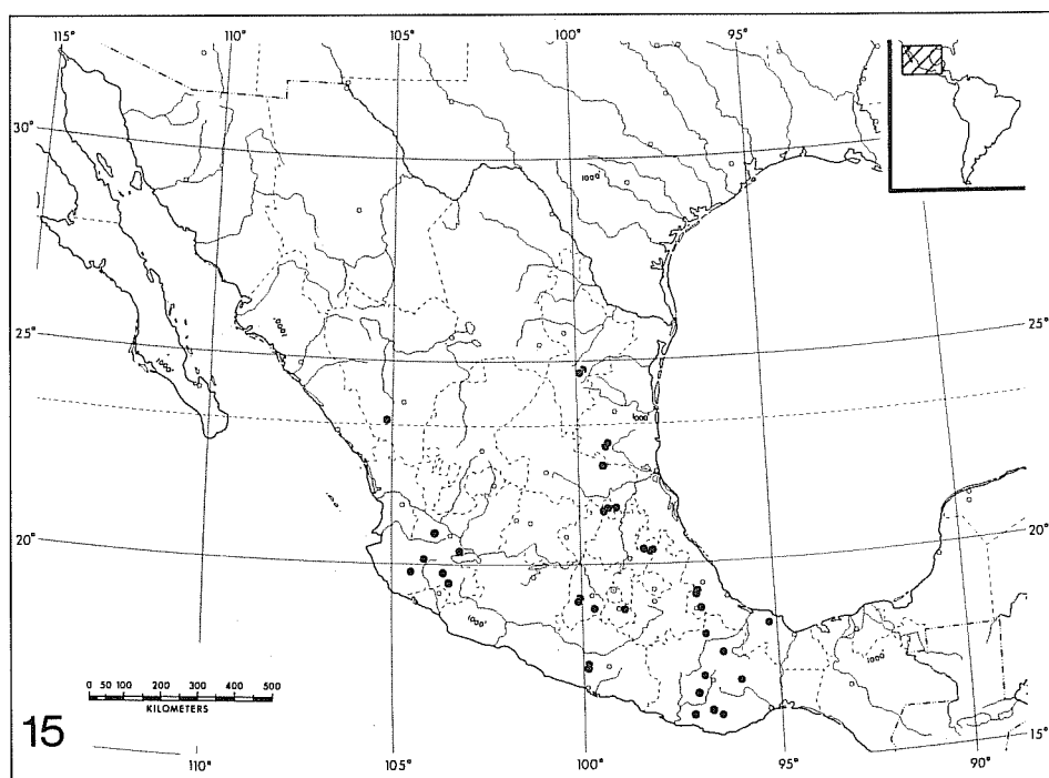
Map 15. Distribution of Nicrophorus olidus in Mexico.
