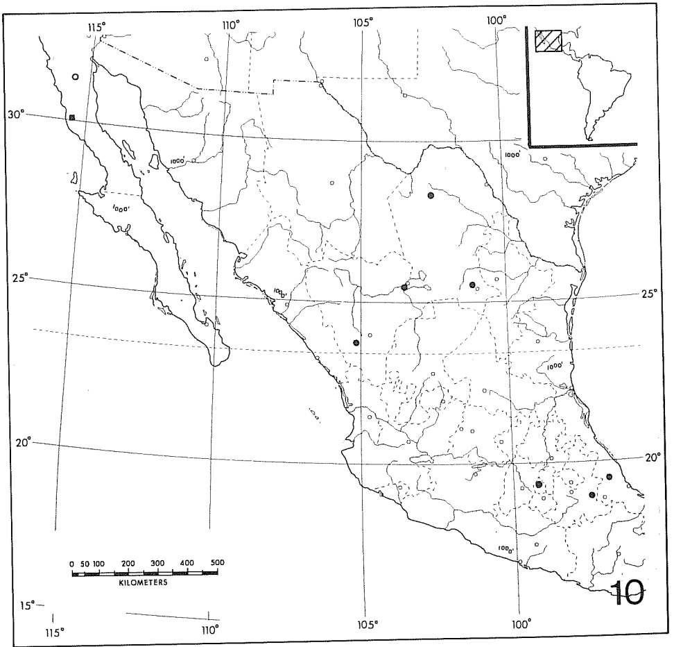
Map 10. Distribution of Nicrophorus marginatus (black dots), Nicrophorus guttula (open dot), and Nicrophorus nigrita (black square, Guadelupe Island record not shown) in Mexico.
