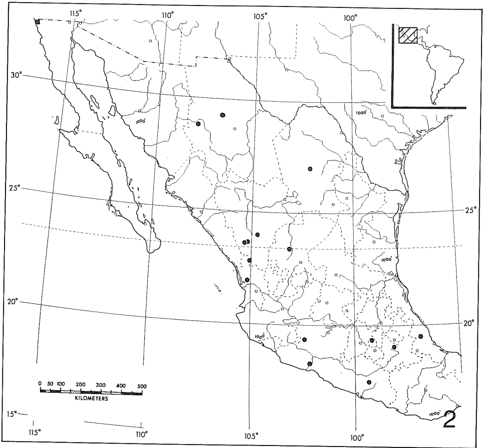
Map 2. Distribution of Thanatophilus truncatus (black dots) and Thanatophilus lapponicus (square) in Mexico.
